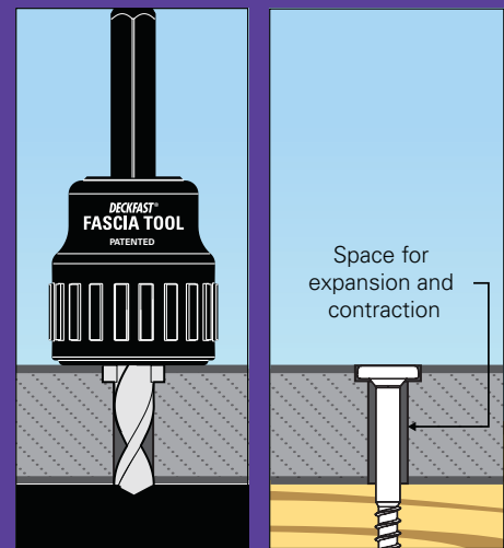
1 Pre-drill with Fascia Tool
