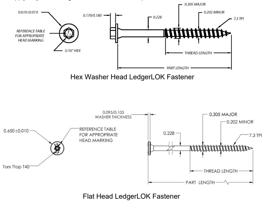
FIGURE 3—LEDGERLOK FASTENERS
