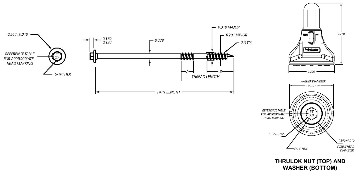
FIGURE 6—THRULOK FASTENER
