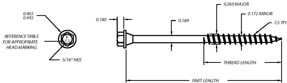
FIGURE 1—OLYLOG/TIMBERLOK FASTENER
