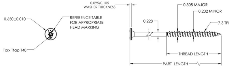
FIGURE 4—VERSALOK FASTENER
