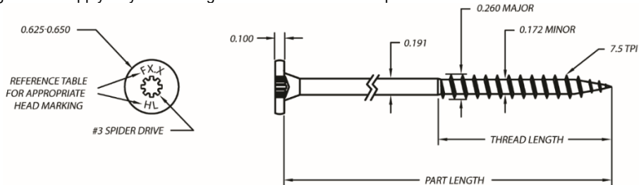
FIGURE 2—HEADLOK FASTENER
