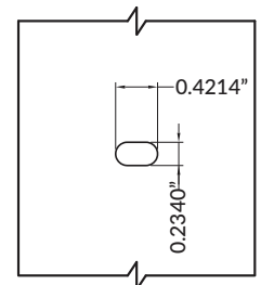
Slot dimensions
